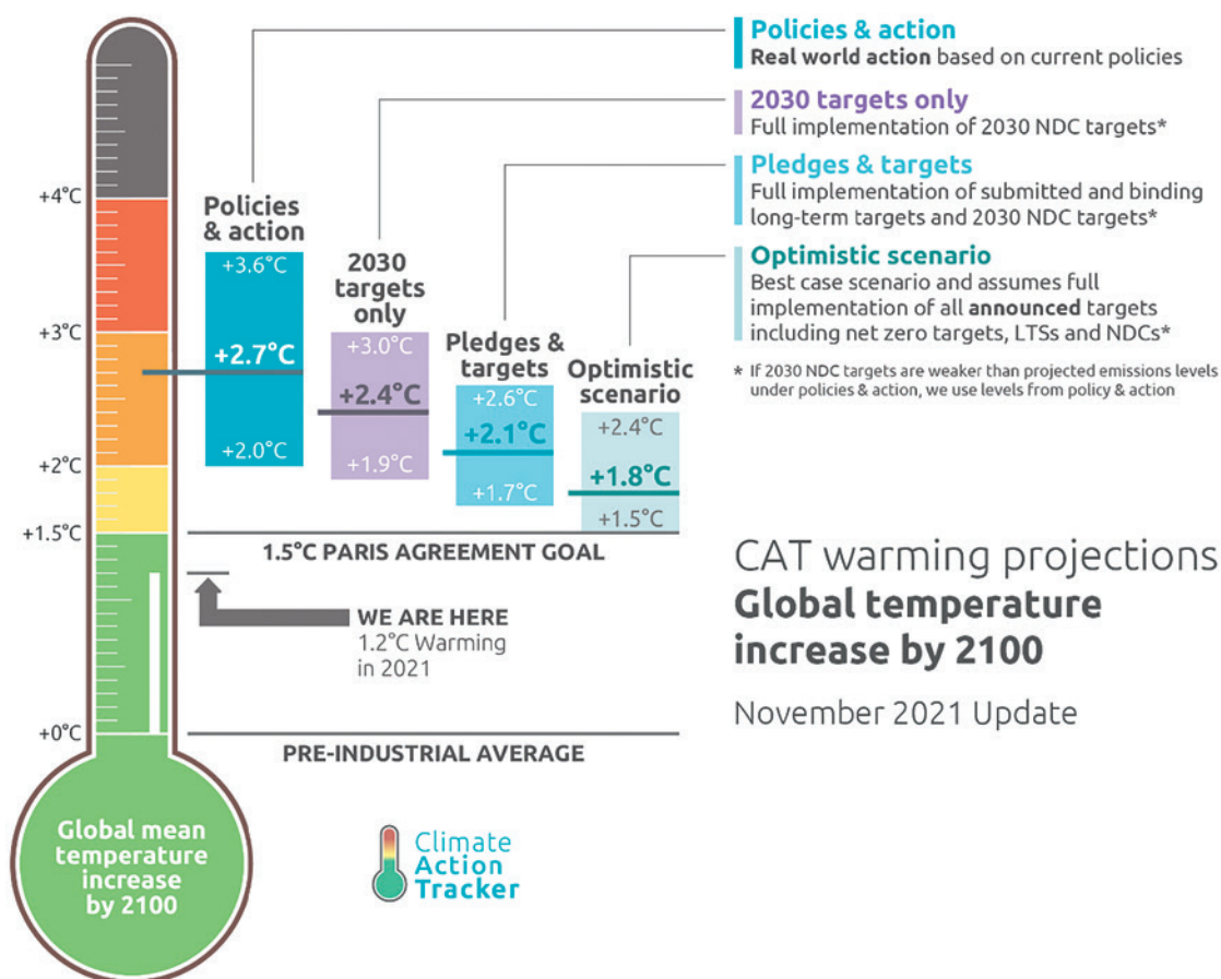
Figure 4 Post-COP26 warming projections. Note, the world is now at 1.2 °C warming, compared with 1.1 °C described by the IPCC report in Box 1. The projections are the median warming estimate in 2100: this means that there is a 50% chance that the calculated temperature would be exceeded if the given emissions pathway is followed; see https://climateactiontracker.org/global/cat-thermometer .
